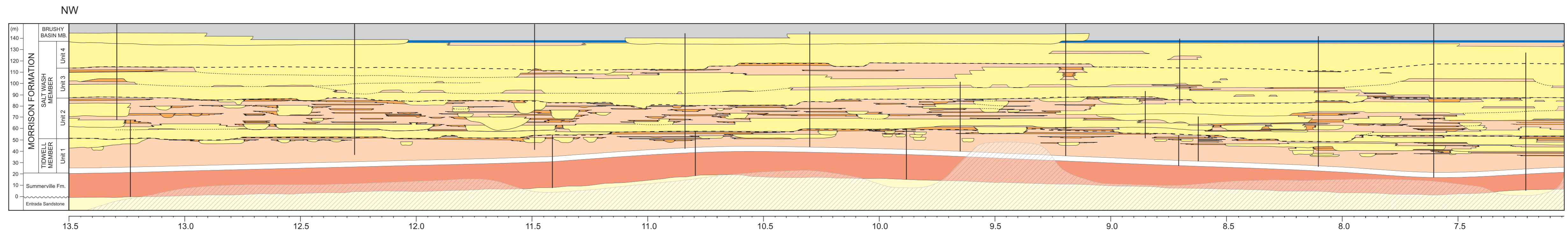
Datashare 28. Cross section of Tidwell and Salt Wash strata mapped along the Waterpocket fold in Capitol Reef National Park, south-central Utah (see Figure 1 for geographic position of the map). The map covers a 150-m (492-ft)-thick stratigraphic interval over a 13.5-km (8.3-mi) distance. The Summerville Formation and uppermost part of the underlying Entrada Sandstone is added at the base of the cross section to illustrate the position of the Morrison Formation relative to older strata. Thick dashed lines indicate the boundaries between correlated chronostratigraphic units (units 1–4). Selected measured sections are indicated on the map as vertical lines. This image can also be seen in an electronic version on the AAPG Web site as Datashare 28 ( www.aapg.org/datashare/index.html ).
